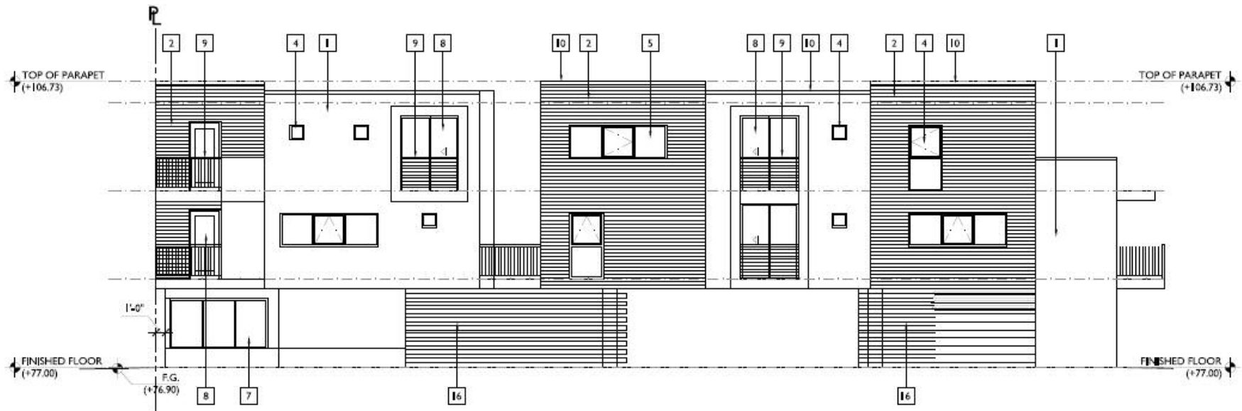
BUILDING B - EAST ELEVATION 02 SCALE: 1/8" = 1'-0"
